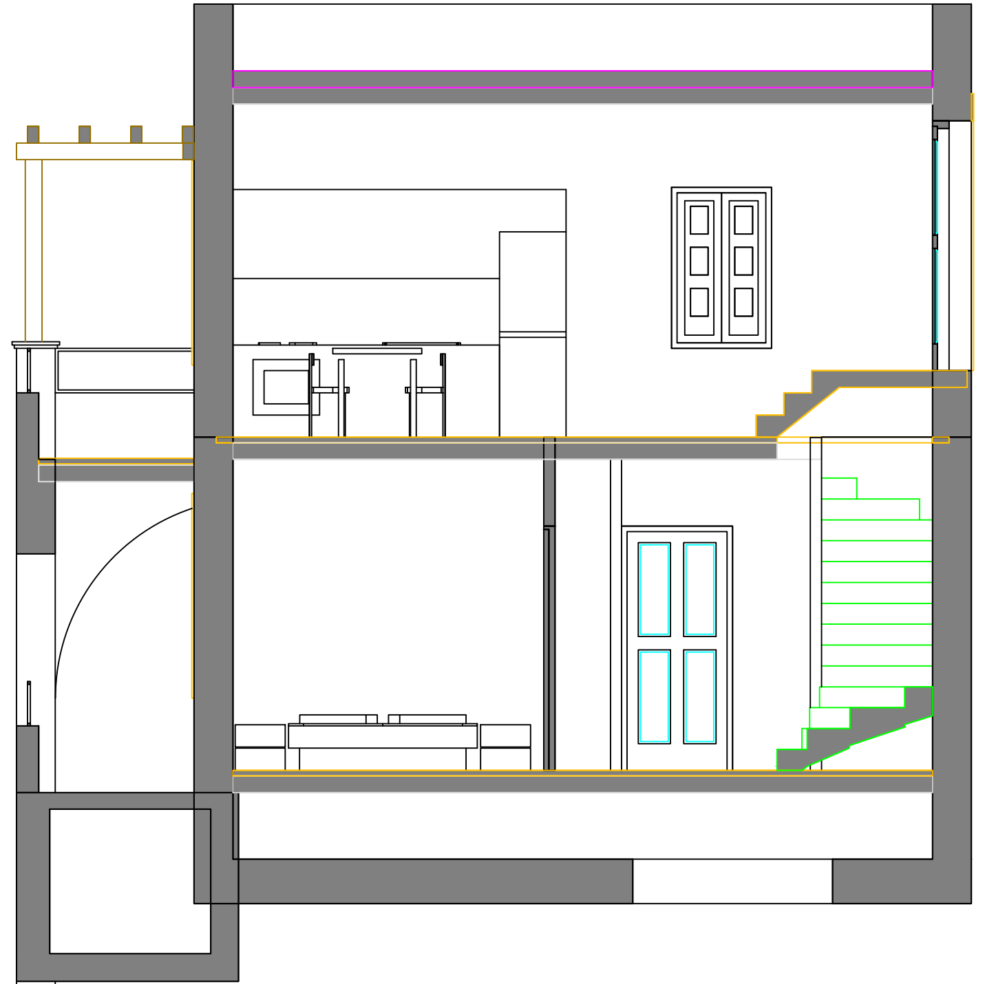
SECTION B
